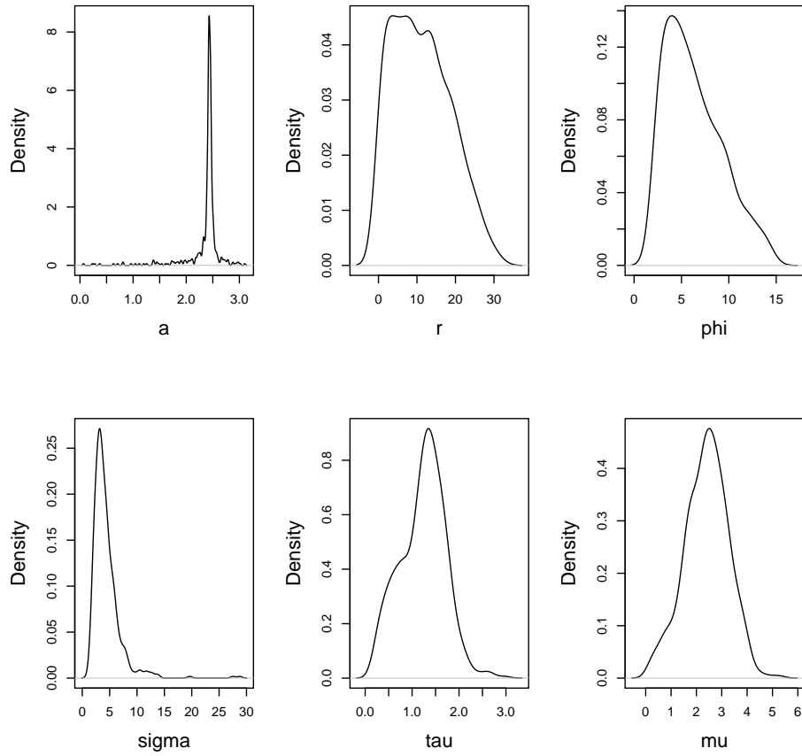
Figure 3: Density plots of posterior samples for all parameters under anisotropy (after burn-in and thinning)
