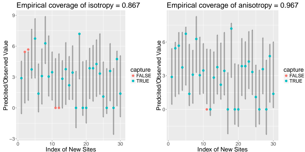
Figure 5: Model comparison: empirical coverage of isotropy and anisotropy
