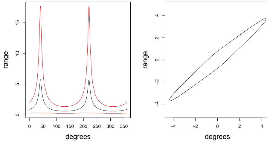
Figure 4: Mean posterior range plotted as a function of angle with associated individual 95% credible intervals. The plot on the right shows the range in polar coordinates which forms an ellipse.
