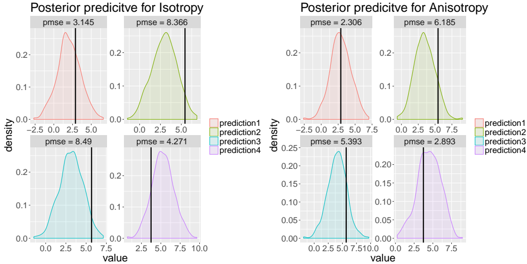
Figure 6: Model comparison: posterior predictive distribution and PMSE for 4 hold out sites under isotropy and anisotropy. Vertical line represents the observed value.
